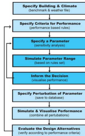
Figure 4 Tool workflow scheme.
